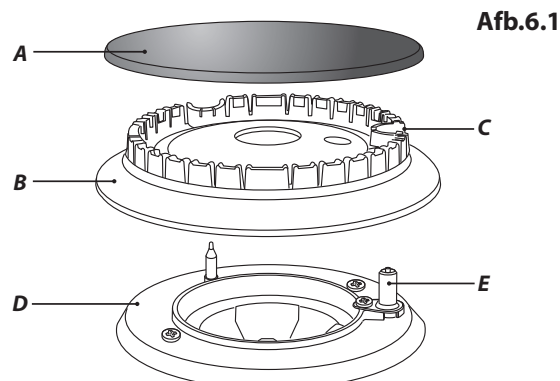
A – Kap, B – Kop, C – Inkeping, D – Basis, E – Elektrode
