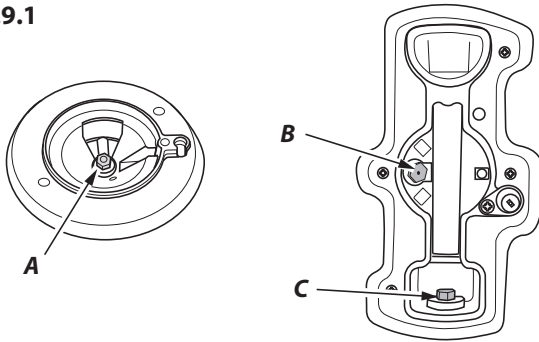
A – Jet, B – Intern injector, C – Extern injector
